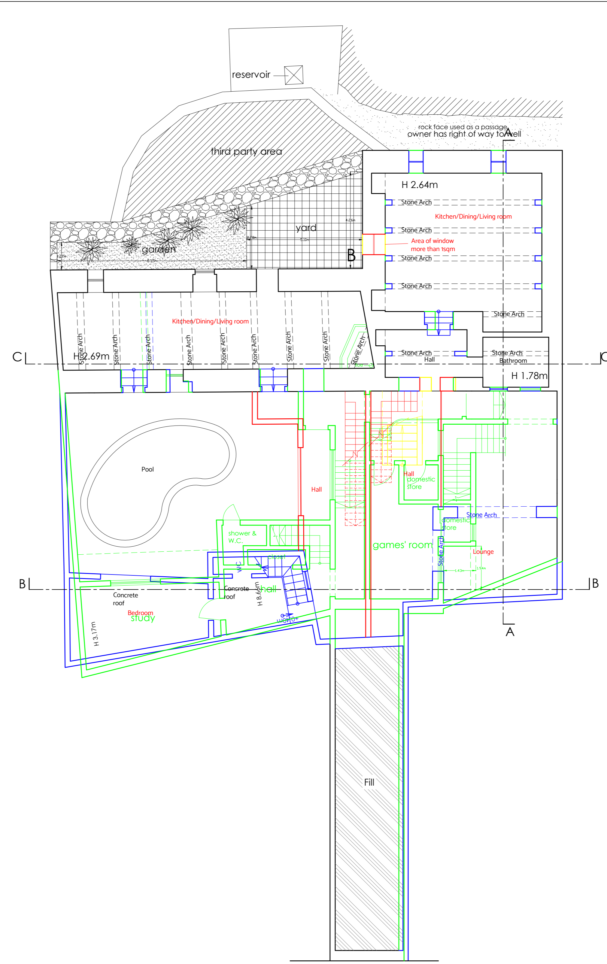
Proposed Basement Level Plan
