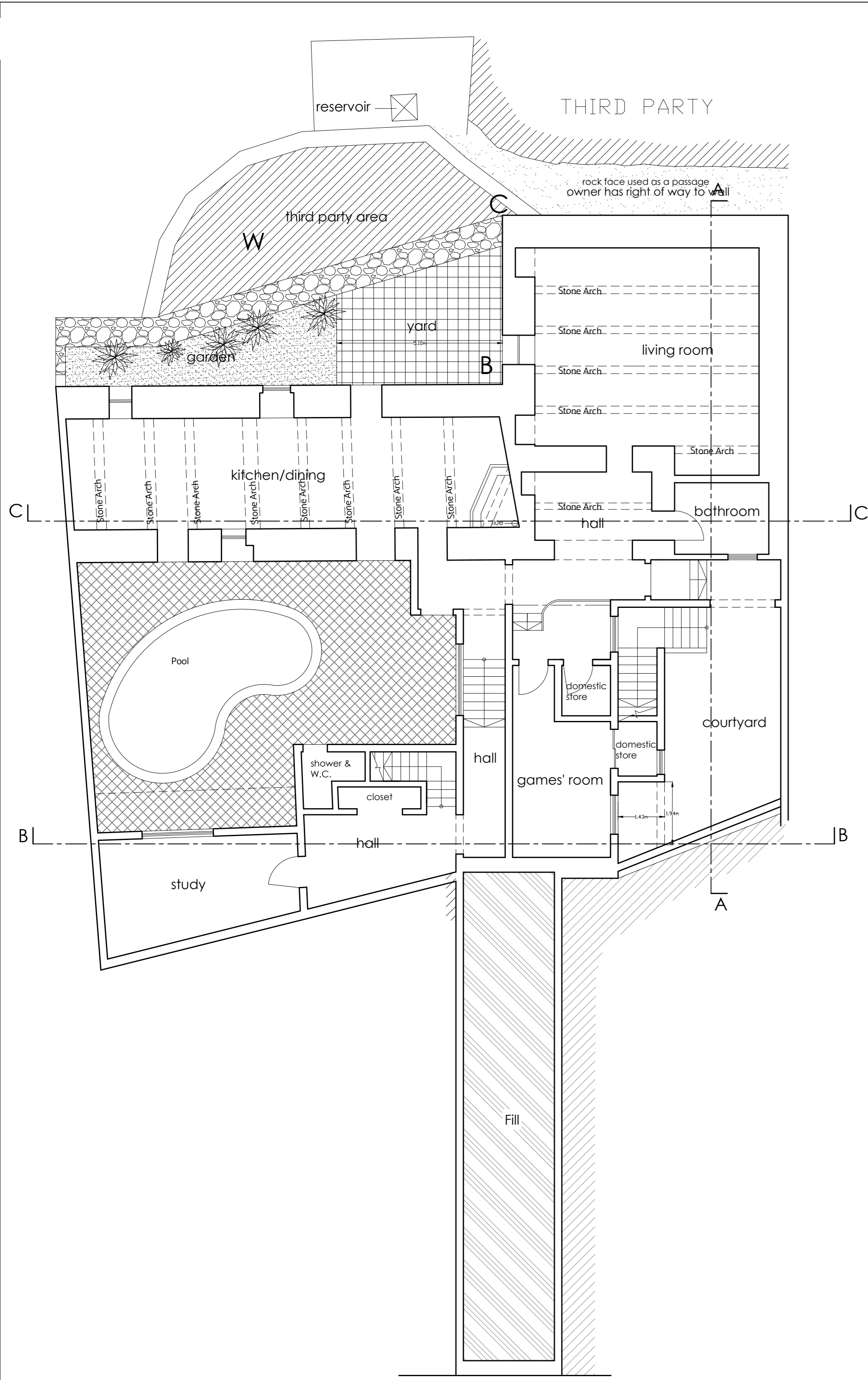
Approved Basement Level Plan
