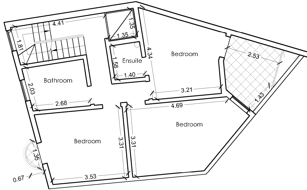
As Proposed First Floor
