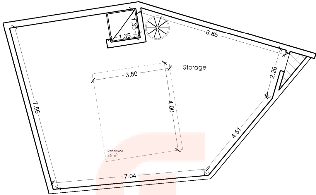
As Proposed Basement Floor
