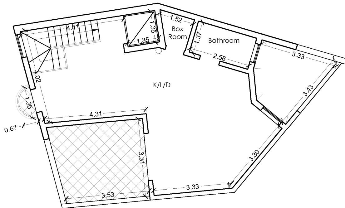
As Proposed Second Floor
