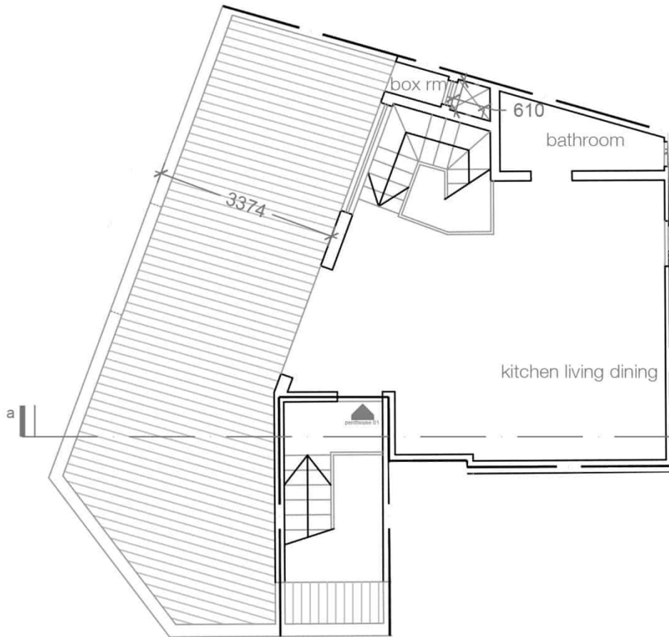
proposed second floor level
