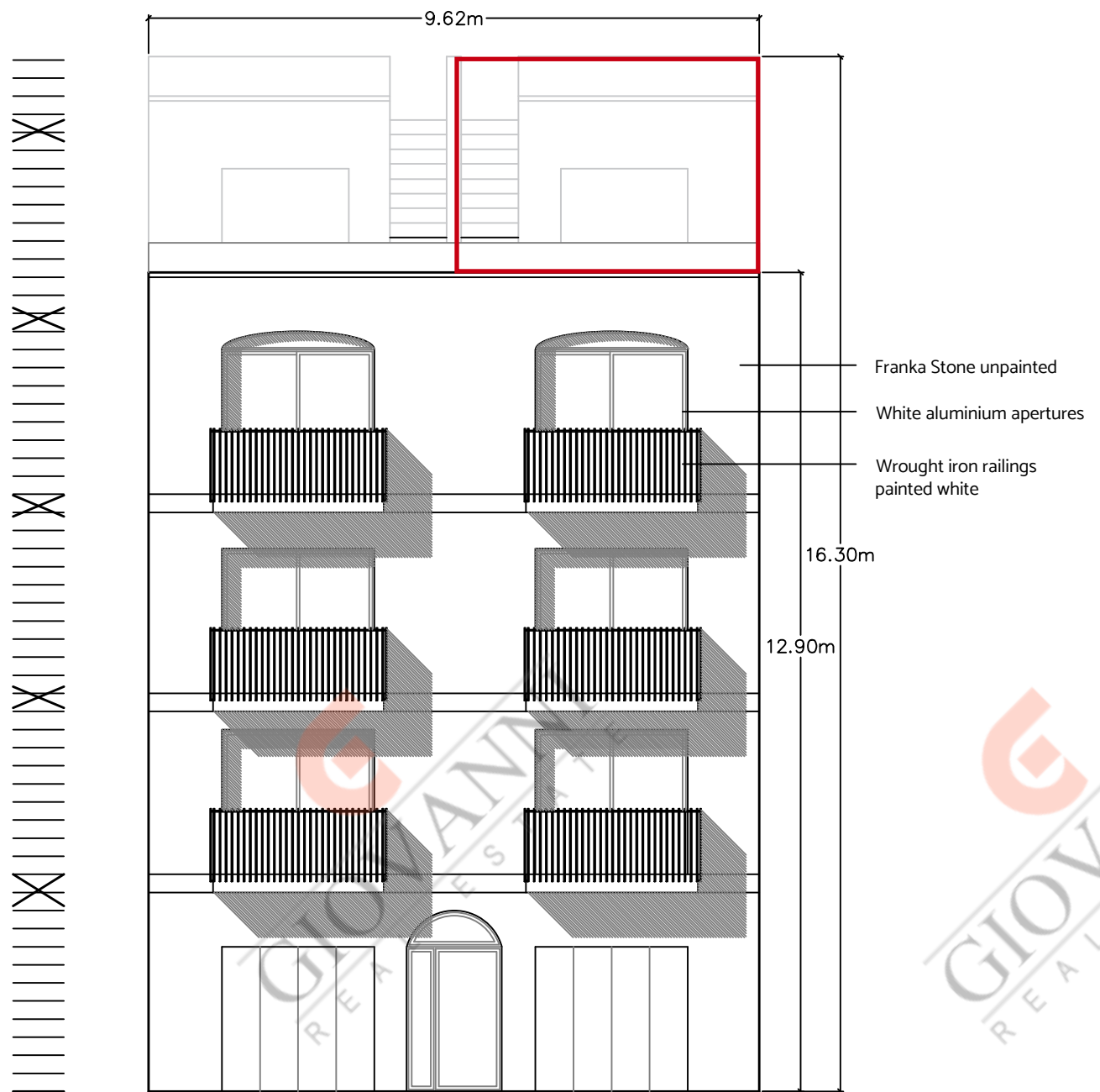
Proposed Front Elevation Scale 1:100 clean copy
