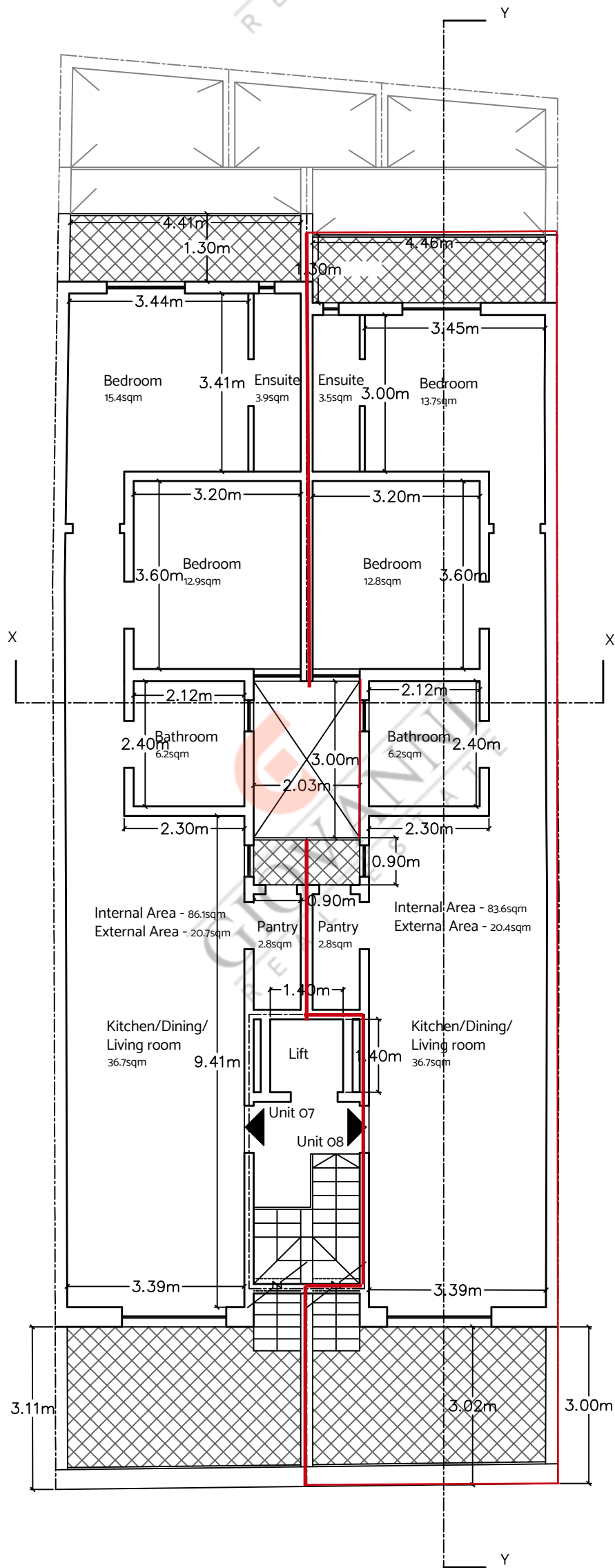
Proposed Receded Floor Level Plan Scale 1:100
