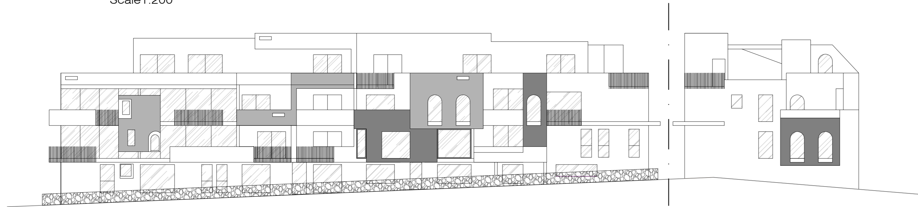
as proposed elevation B
