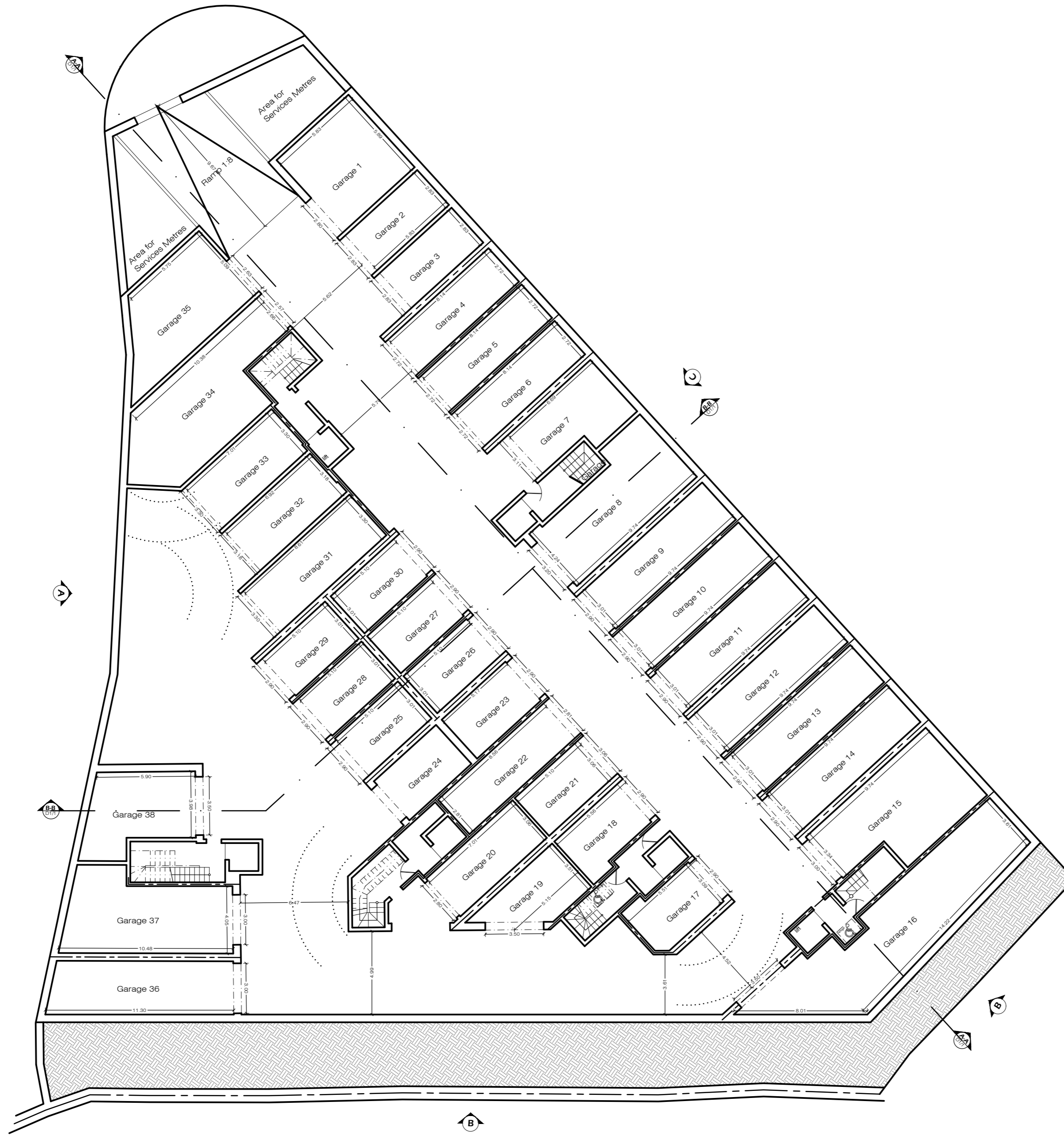
level -1 Scale 1:200
