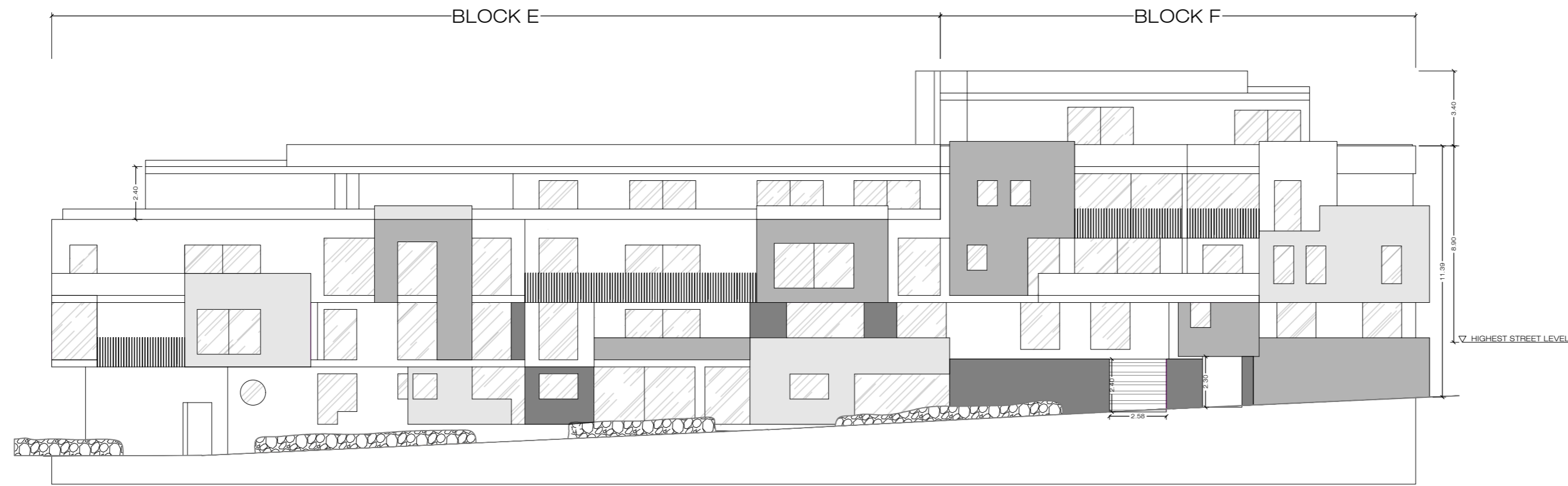
as proposed elevation A
