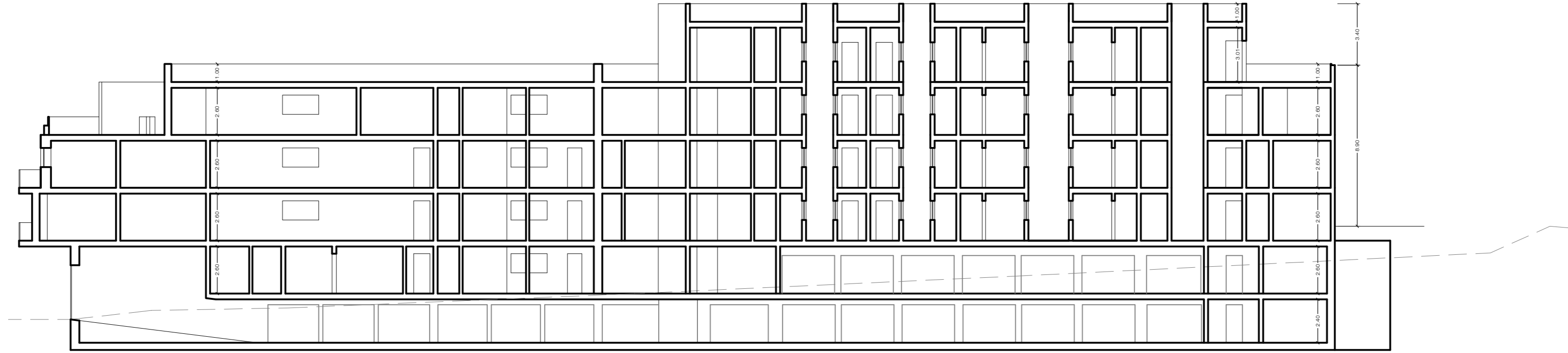
○ as proposed section A-A Scale 1:200
