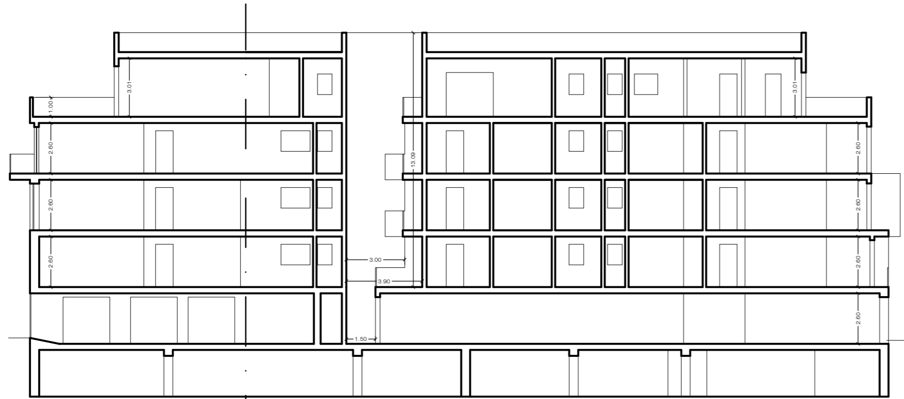
○ as proposed section B-B Scale 1:200
