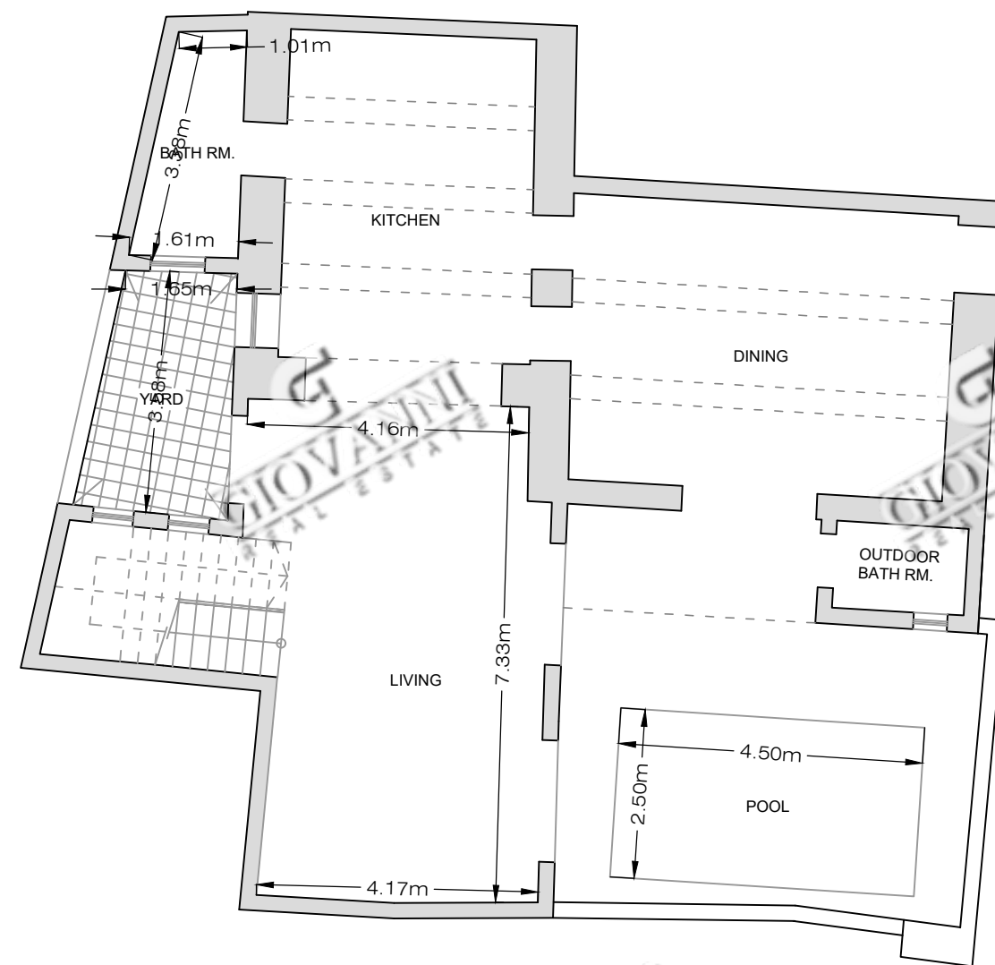
PROPOSED GROUND FLOOR - Clean Copy Scale 1:100
